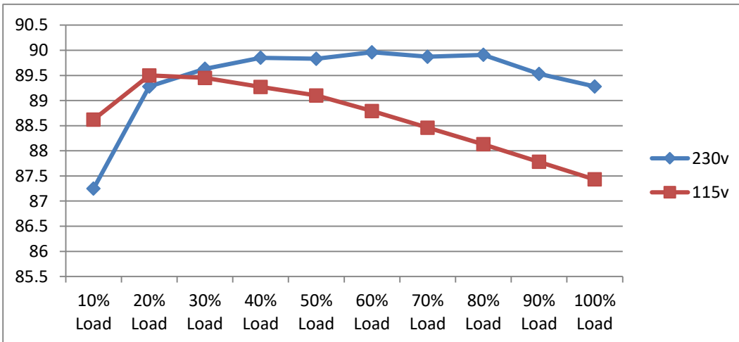
EFFICIENCY vs LOAD
